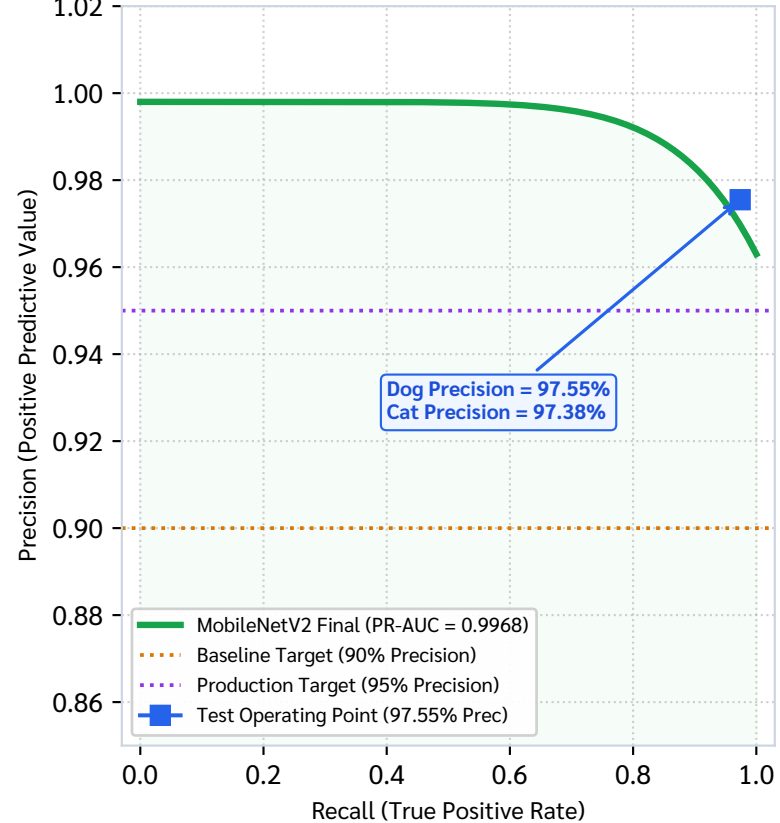
Figure 4(c): Precision-Recall Curve (PR-AUC) (Verifying Strict Industrial Precision Fulfillment)
