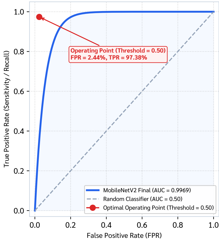
Figure 4(b): Receiver Operating Characteristic (ROC) (Confirming Near-Perfect Class Discrimination)
