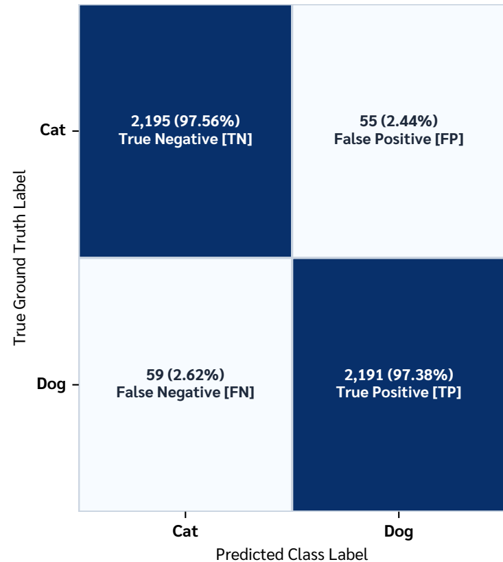
Figure 4(a): Normalized Confusion Matrix (Holdout Test Set, N = 4,500 Images)
